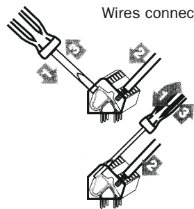
Wires connection to terminal block
